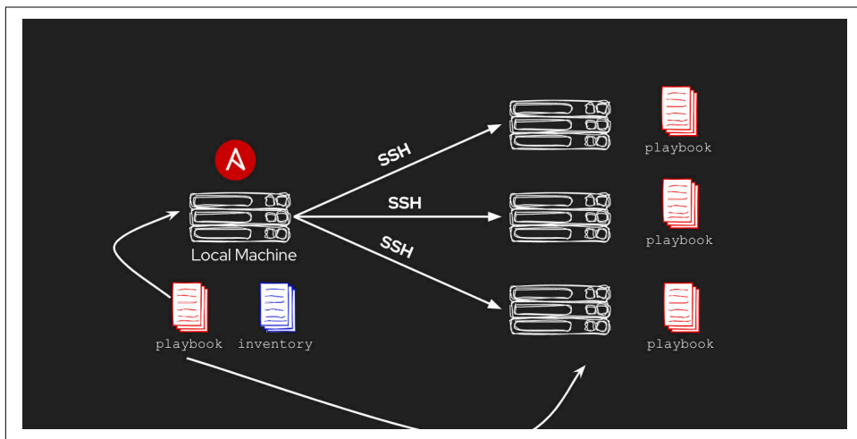
Figure 2-2. Control node copies modules to managed nodes
